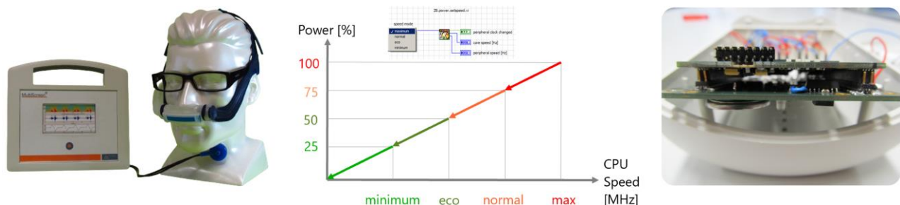
Fig. 22 | Low power consumption was the be-all and end-all for this mobile measuring device. This was achieved by switching off unused components or scaling the processor clock.
